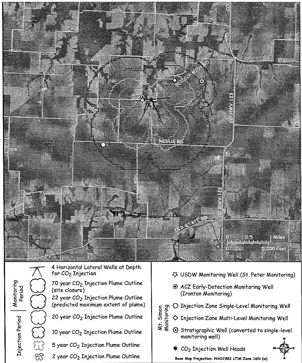
Figure 1. Monitoring Well Network as Presented in Testing and Monitoring Plan (Chapter 5.0) of UIC Permit Supporting Documentation as Submitted in May 2013
